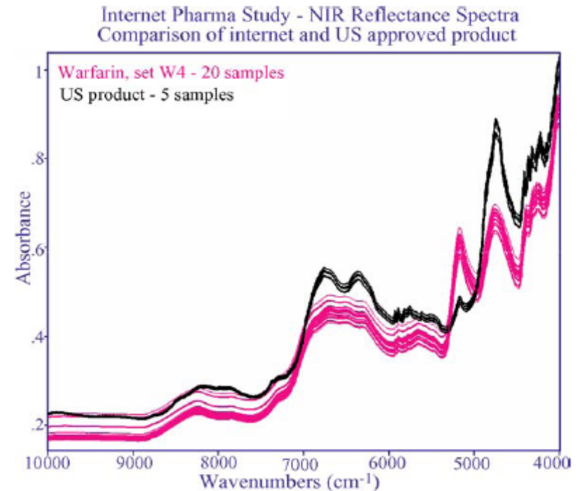
Fig. 8. NIR spectra of warfarin sodium products. NIR of warfarin sodium: more variability is seen with the internet product (pink) than the U.S. product (black). The difference in peak intensities suggests the same formulation but in different proportions.
