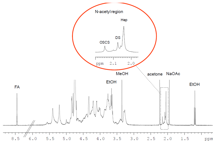
Chondroitin sulfate A/C Galactosamine + Glucuronic acid R = R' = sulfated
